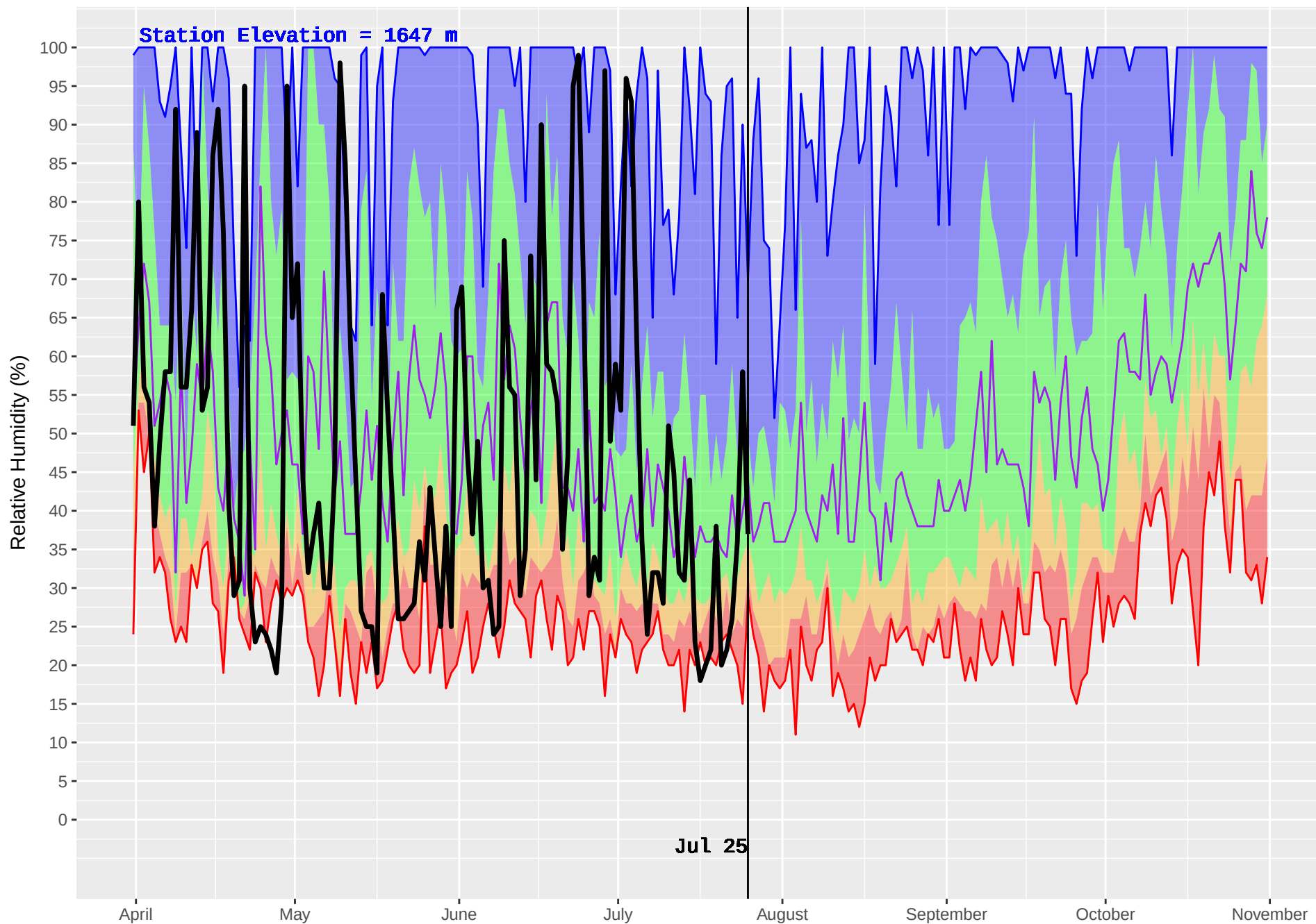
ROUND PRAIRIE (788) : Historical (2001–2016) and Current (2018) Noon Relative Humidity
