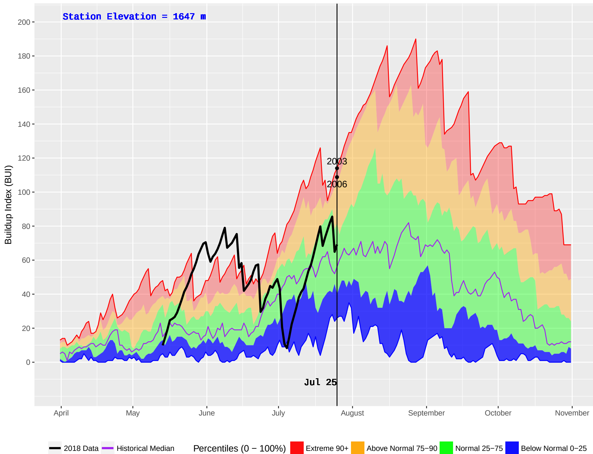
ROUND PRAIRIE (788) : Historical (2001–2016) and Current (2018) Noon Buildup Index (BUI)
